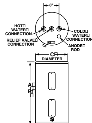
WATER CONNECTIONS ALL 3/4" N.P.T.
